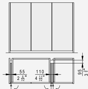
Door striking against the top and bottom cabinet sections
