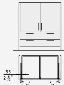
Composed cabinet overlay doors
